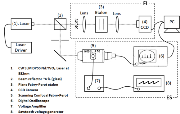
Fig. 2: The experimental setup for the characrerisation of the Nd:YVO 4 Laser.
