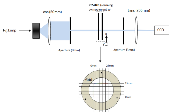
Fig. 6: Experimental setup for the characterization of the Fabry-Perot etalon with respect to its Flatness.
