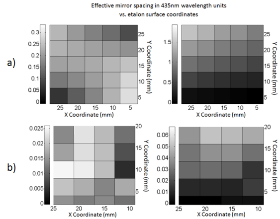
Fig. 7: a) Prototype 13 mm etalon b) Commercial 5 mm etalon. Left: Map of the effective etalon spacing (in units of 435 nm wavelength) with deviation from parallelism removed to reveal the etalons flatness. Right: Map of the effective etalon spacing.
