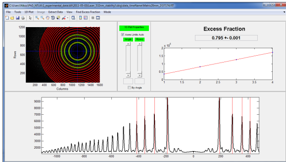
Fig. 1: MATLAB Program for the analysis of interference fringe images.
