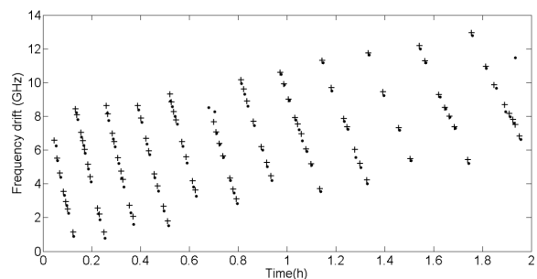
Fig. 3: Plot of the frequency drift vs the elapsed time from the moment the laser started to operate.
